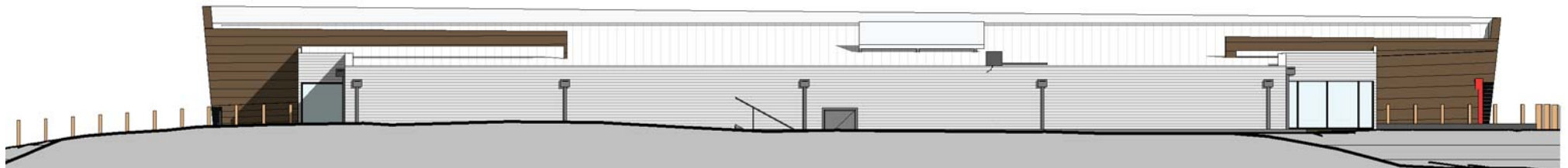
PROPOSED ELEVATIONS - REAR VIEW
